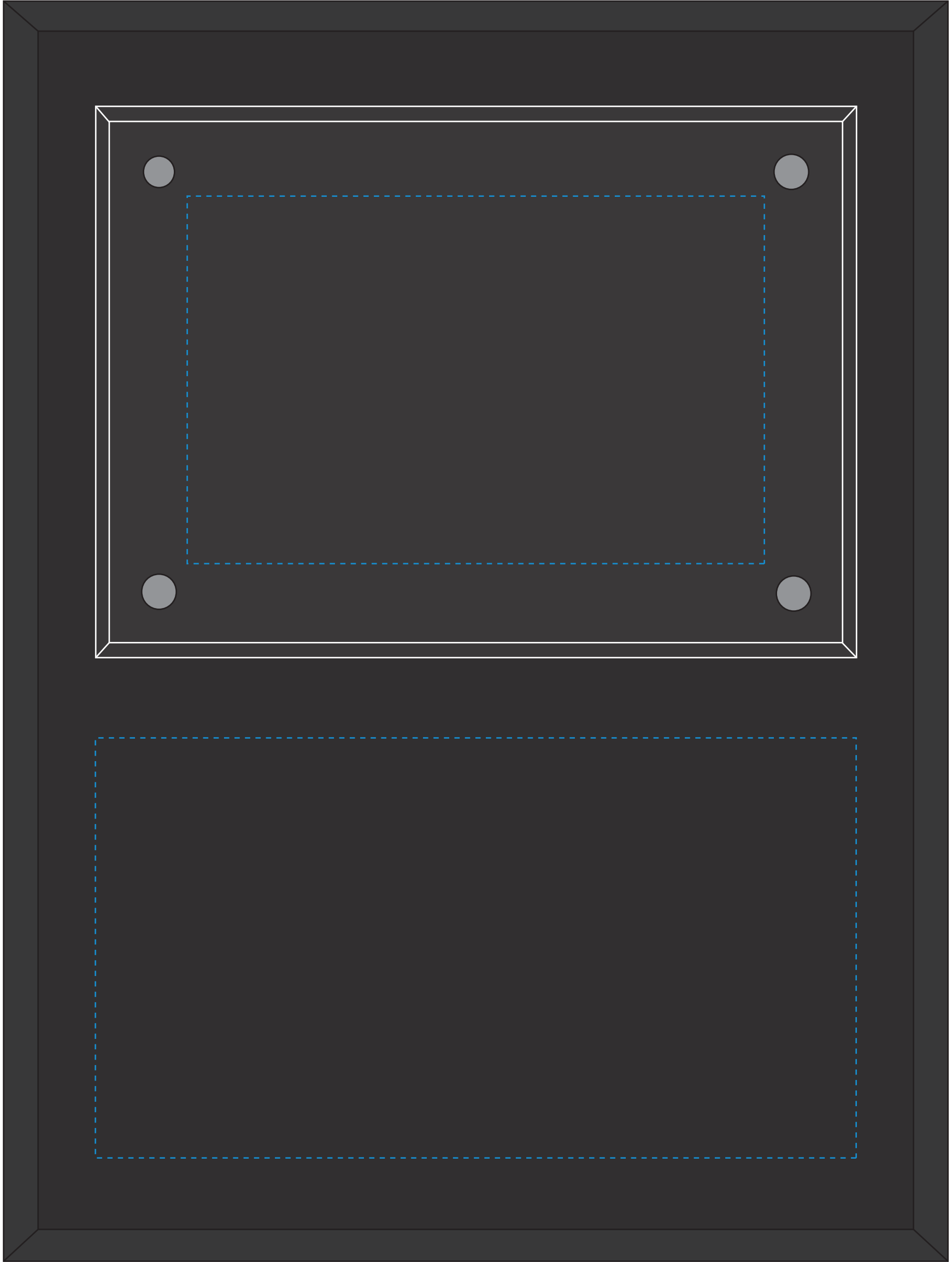
6582 BAJA BLACK PLAQUE - 9" X 12" Laser Front ON PLAQUE Blue line represents the max image area.
